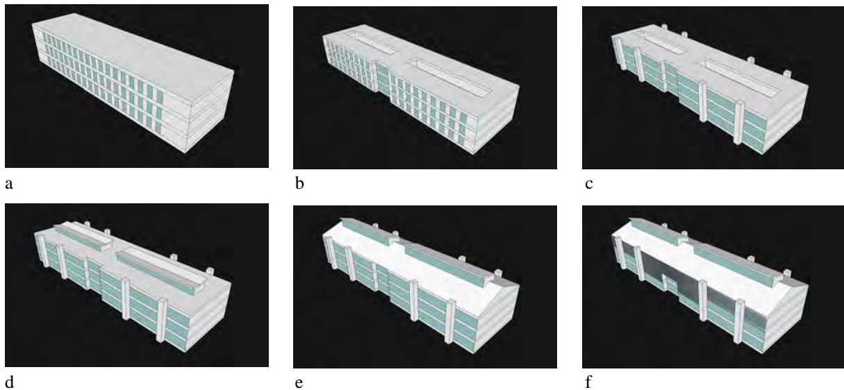
Figure 5: A selection of the various design models explored: a) floor to ceiling height of 4.5 metres; b) floor to ceiling height of 3.5 metres with central unenclosed atria; c) addition of cooling towers; d) enclosed central atria; e) roof pitch of 23°; f) addition of window shading.
